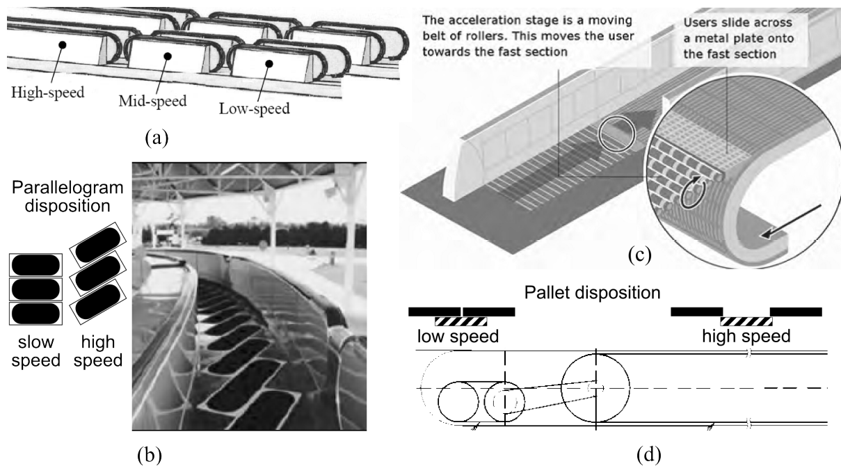
Figure 4. Accelerating moving walkway types. (a) in-line belts, adapted from Loder (1998). (b) sliding parallelograms, adapted from Todd (1974). (c) accelerating/decelerating rollers, adapted from Cote and Gempp (1998). (d) sliding pallets, adapted from Gonzalez Alemany and Cuello (2003).
