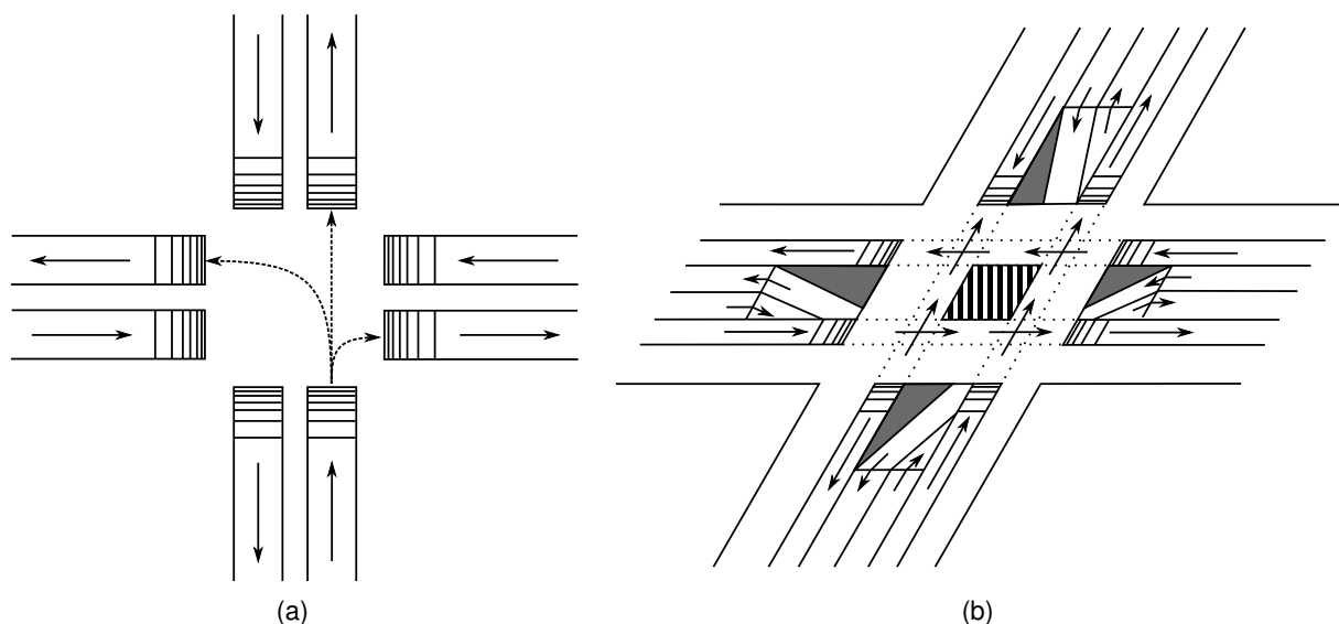
Figure 3. Possible intersection designs: (a) single-layer intersection and (b) multiple-layer intersection with expressways. Adapted from Rojanawisut (2015).
