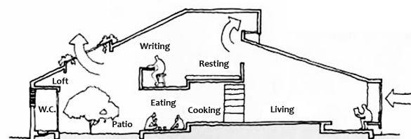
Section (during day)
